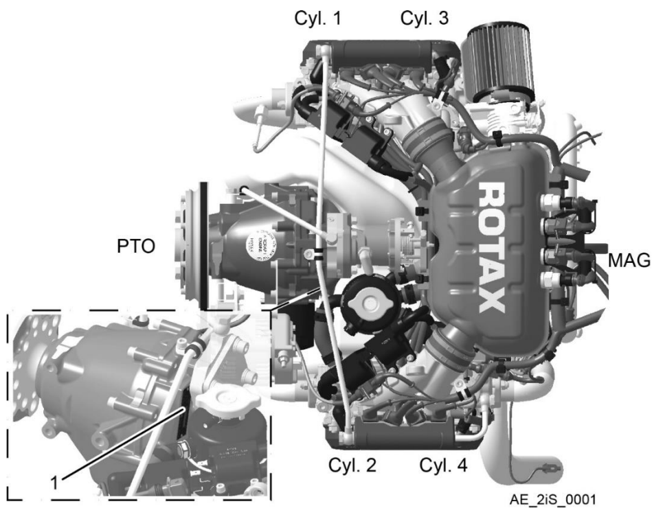
Figure 1.2: Engine
